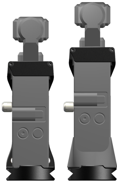
EXO Pocket Cage is compatible with the original DJI Pocket wireless base add-on.
